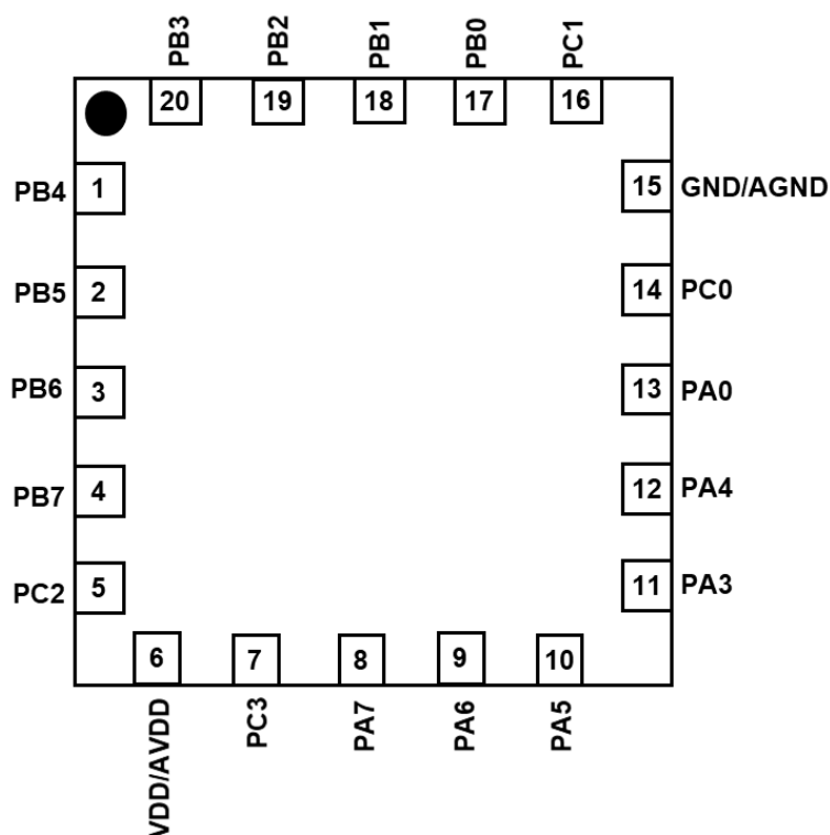
PFS123-1J20A: QFN3*3-20P
