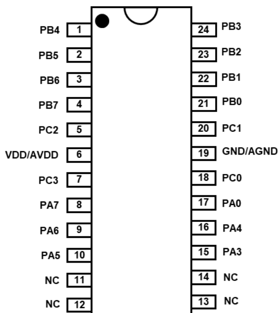
PFS123-Y24: SSOP24(150mil)
