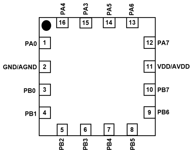
PFS123-1J16A: QFN3*3-16P (0.5pitch)
