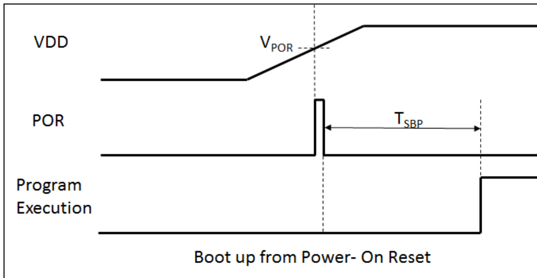
Fig.1: Power-Up Sequence
