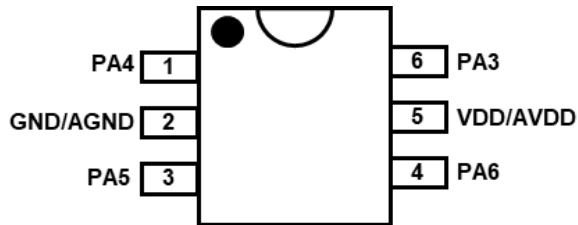
PFS123-U06: SOT23-6 (60mil)
